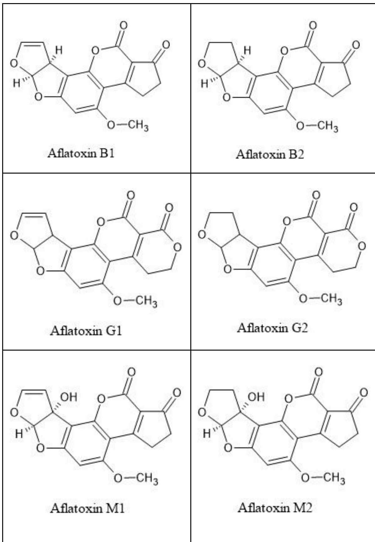
Figure 1: Chemical structure of different types of aflatoxin
